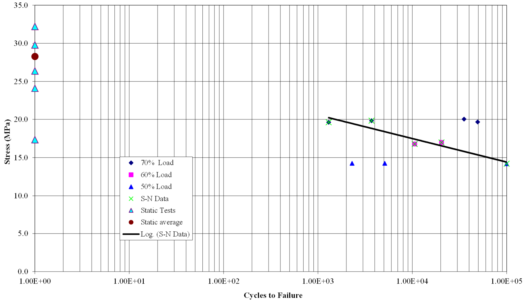
Flatwise Tension Fatigue S-N Curve @ 50°C CTD-425/S2 Glass with Copper substrate and CTD-450 primer
