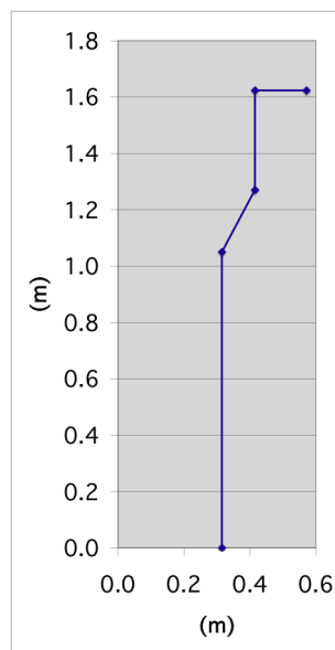
Figure 3-1 - Line Segments Defining Plasma Facing Surfaces
