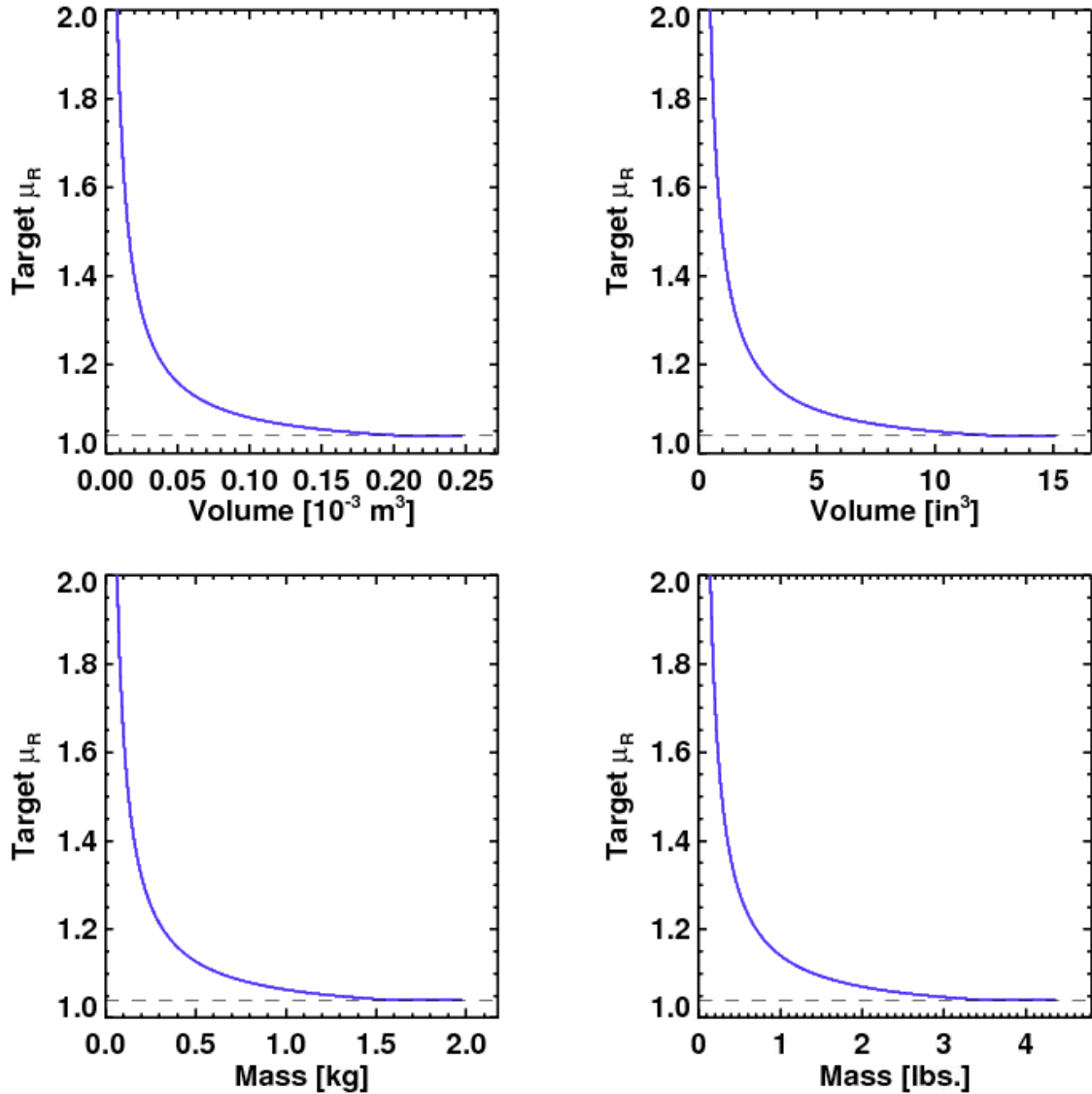
Figure 2-3: Target \mu_R and object sizes that result in a 1 G midplane separatrix magnetic perturbation, for a typical NSTX-Upgrade equilibrium and object position of Z=0, R=1.65 . Masses greater than 1.5 kg have a target base material permeability of 1.04.
