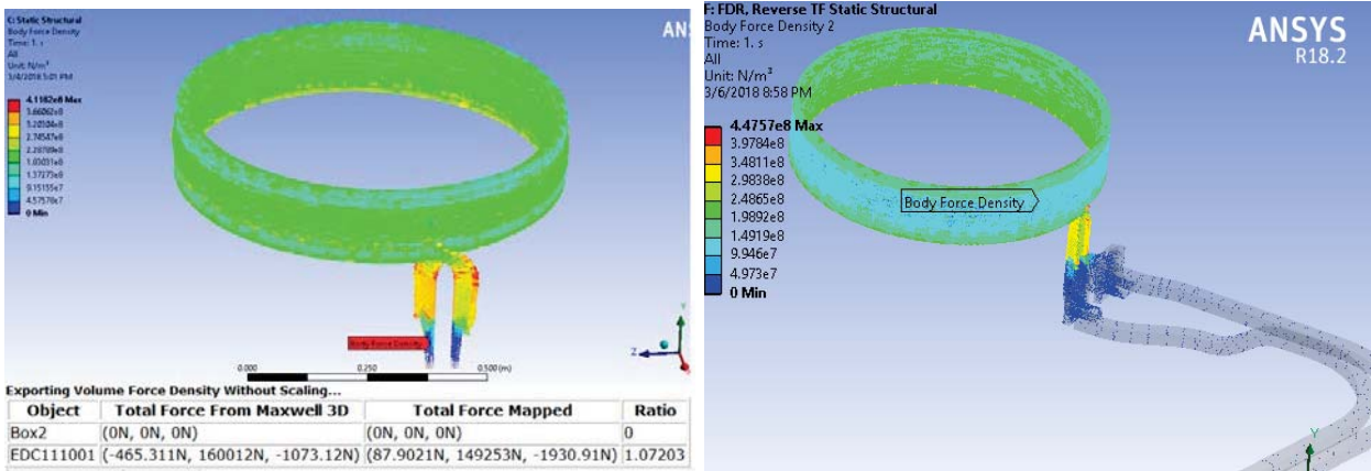
Figure 9 Mapped force densities for PF-1a, 1b upper assembly and PF-1b lower
