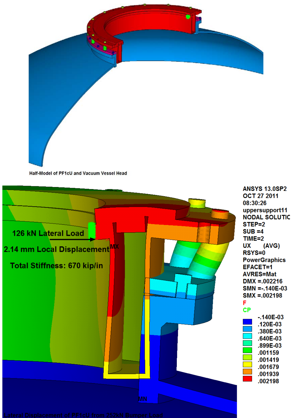
Fig. 4.5-2 PF1a/bU & Center Casing, Lateral Displacement from -252/2 kN Bumper Load
