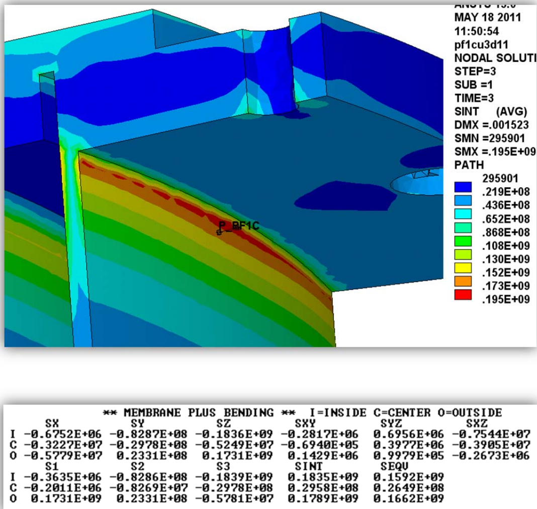
Fig. 4.4.3-3 PF1c 3D model Stress contours and Linearized MEM+BEND Stress
