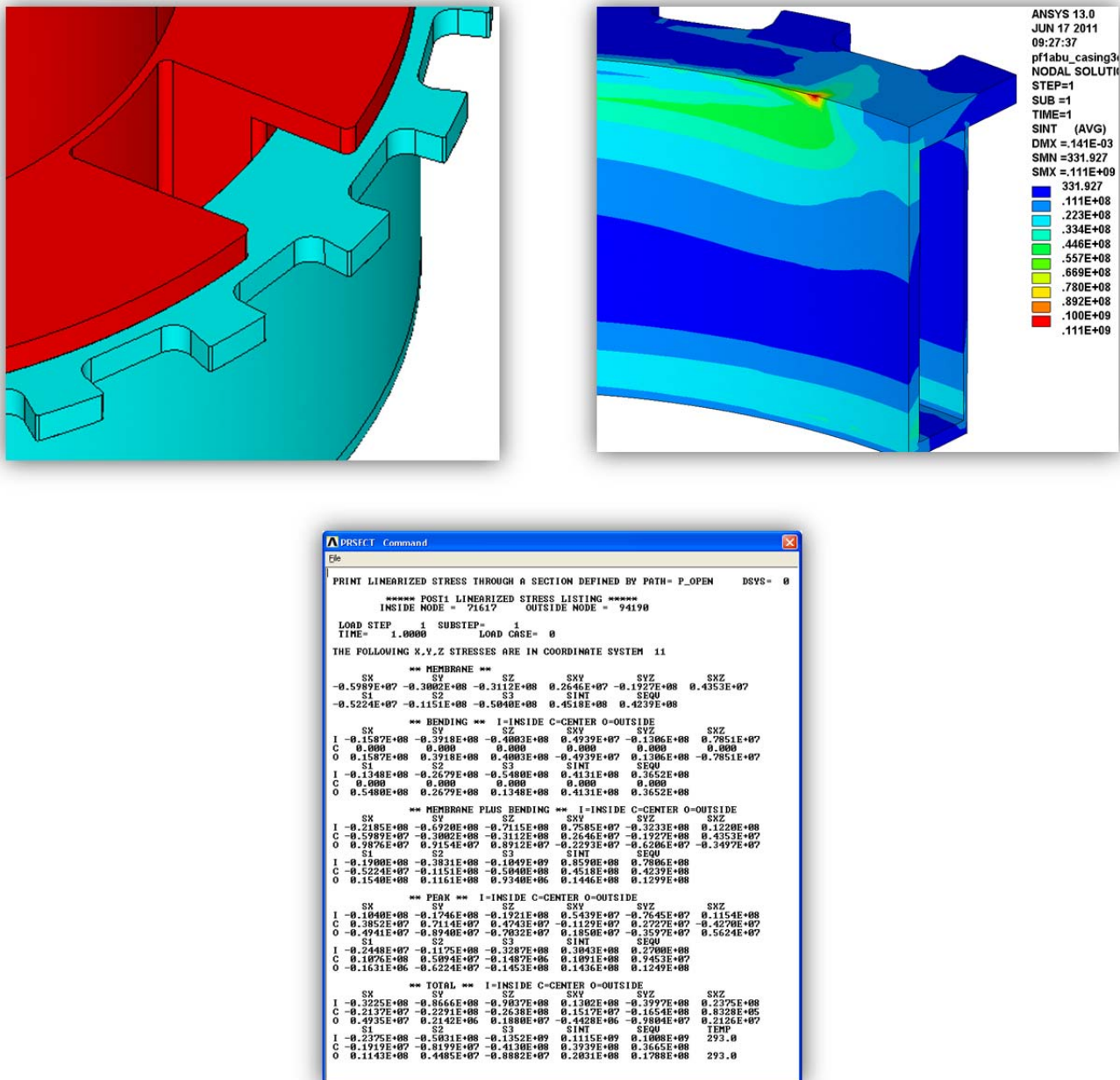
Fig. 4.4.1-5 Close-up view (top-left), Tresca Stress (top-right) and Stress Categorization (bottom)
