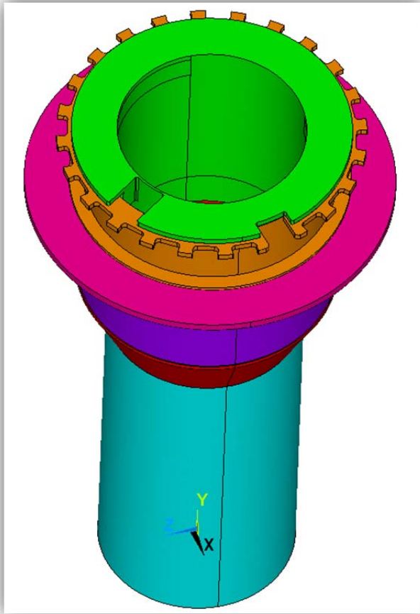
Fig. 4.0-4 Examples of 3D Modeling Details
