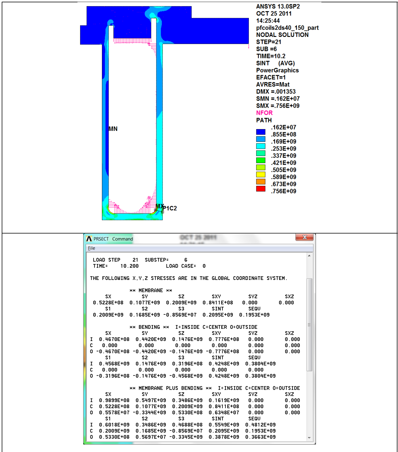
Fig. 4.3.11-9 Tresca stress and Linearization, PF1c structure (EQ10, WP at 100°C)
