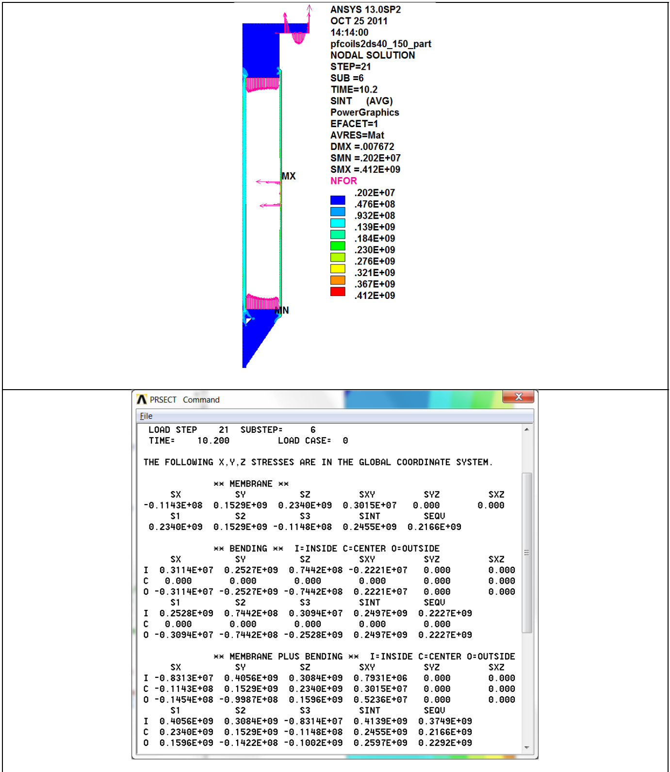
Fig. 4.3.11-7 Tresca stress and Linearization, PF1a structure (EQ10, WP at 85°C)
