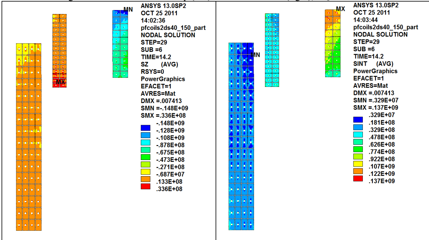
Fig. 4.3.11-5 PF1a/b/c Cu Hoop (left) and Tresca Stress (right), EQ14 EM + Thermal
