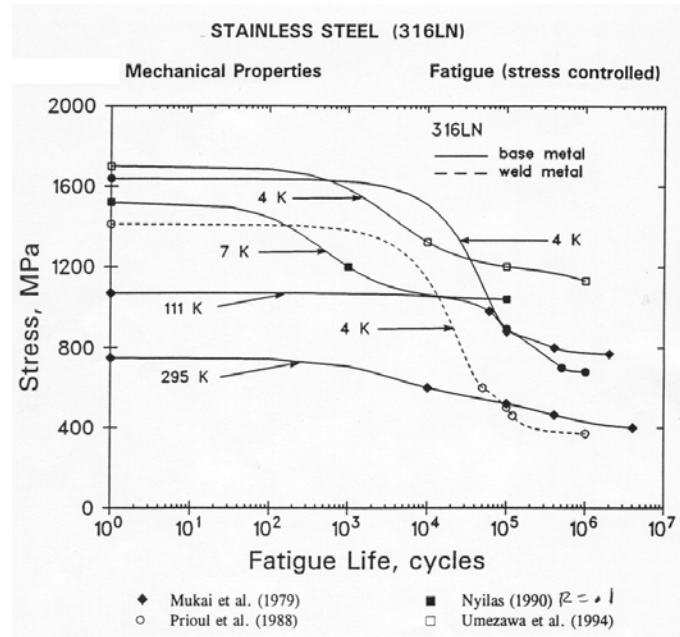
Figure 3.3-1 Fatigue S-N Curve for 316 Stainless Steel
