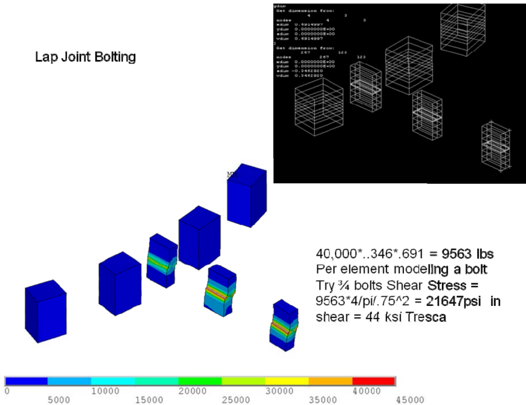
Figure 6.1-6 Lower Flat Spoked Lid Lap Joint Bolting.
