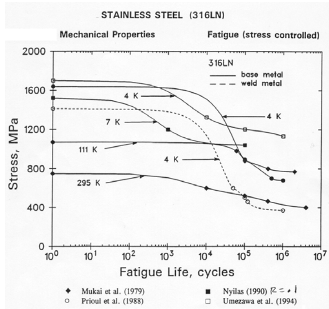
Figure 7.0-3 Fatigue S-N Curve for 316 Stainless Steel
