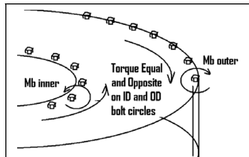
Figure 2 Torques and Moments
