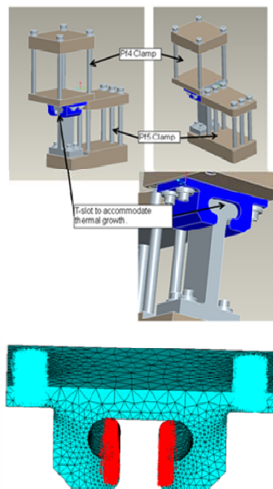
Figure 12.6-2 Dovetail Stress Analysis
