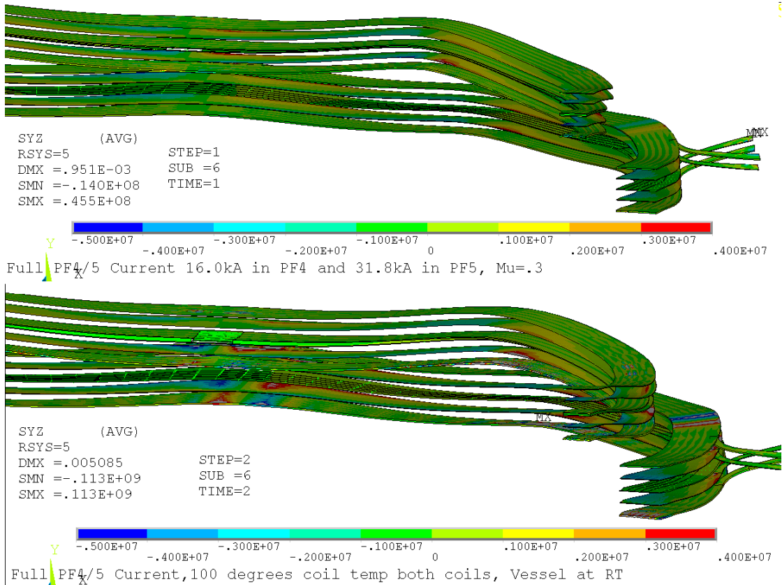
Figure 8.3-3 Radial -Vertical Shear for Lorentz and Lorentz plus Both Coils Hot
