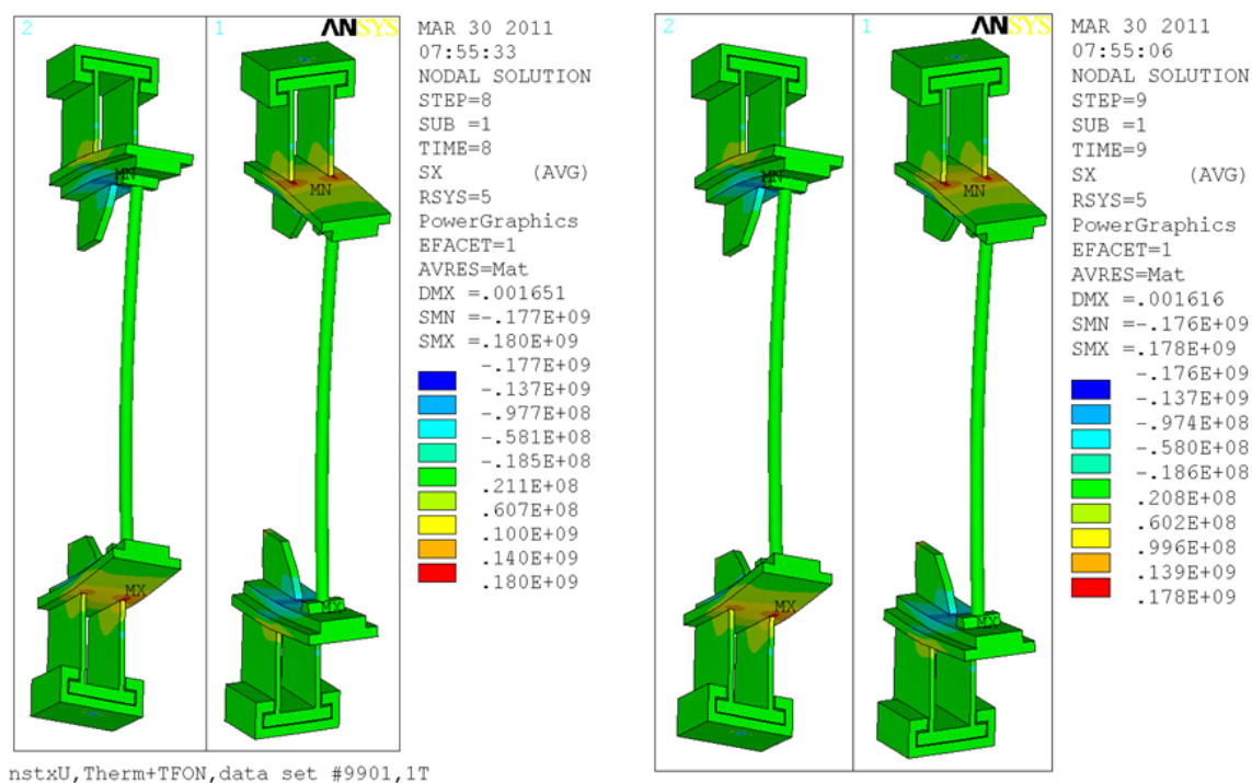
Figure 12.3-5 Existing Support Bracket - With Strut, EQ 01 and EQ 02
