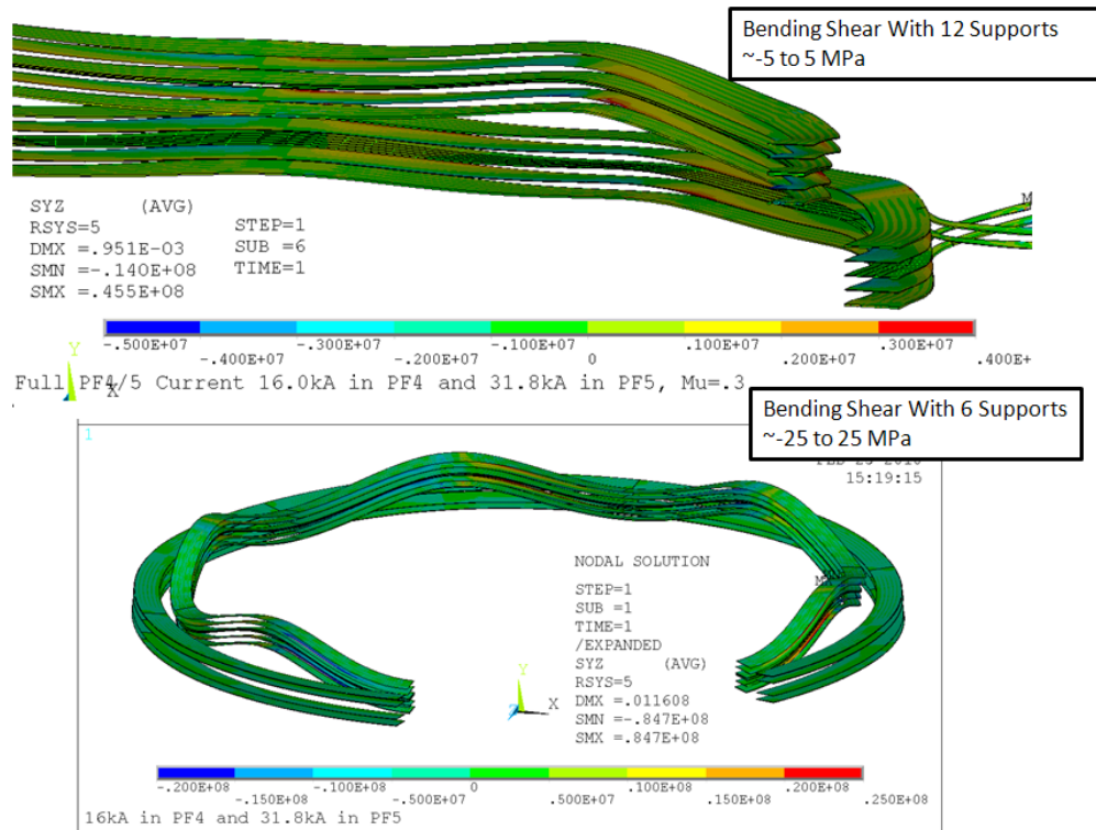
Figure 8.3-4 Radial -Vertical Shear for Lorentz Only, Full Coil Currents
