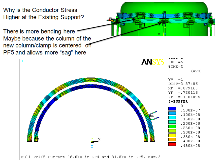
Figure 9.1.1-14 Effect of New Column Position
