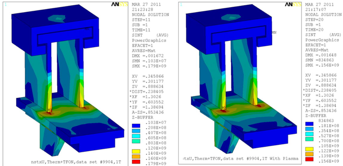
Figure 12.3-4 Existing Support Bracket - No Strut, EQ 04 With and Without Plasma
