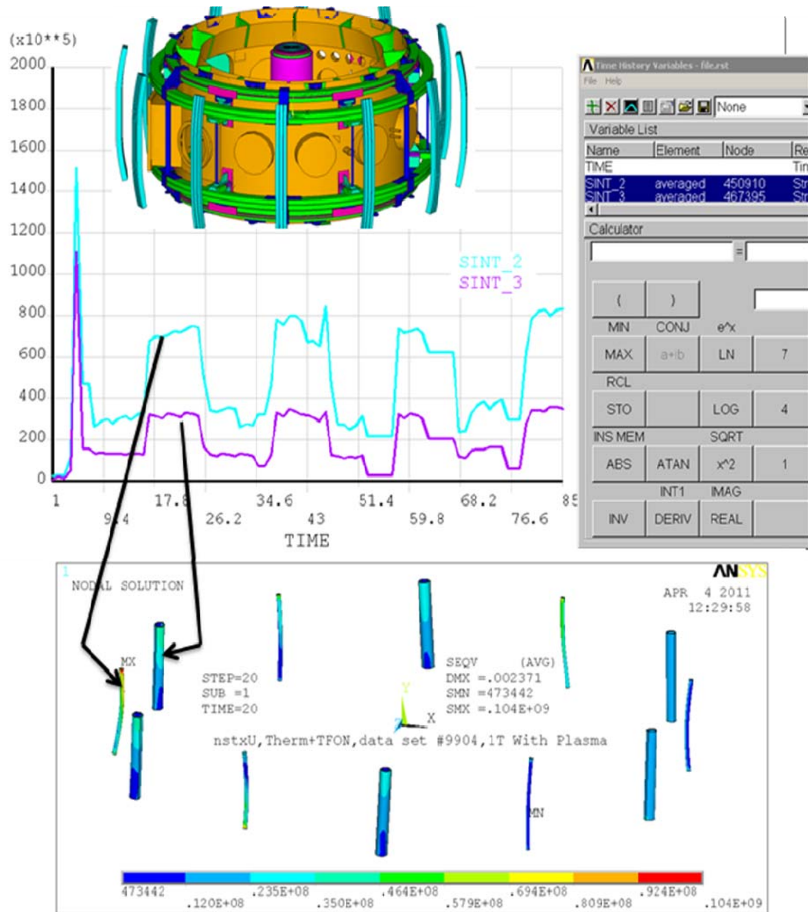
Figure 12.4-1 Column Stress From Global Model (Original Existing thin Column)
