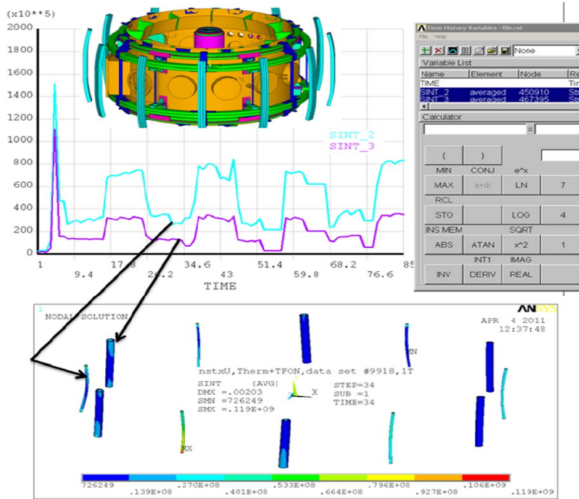
Figure 12.4-2 Column Stress From Global Model (Original Existing thin Column)
