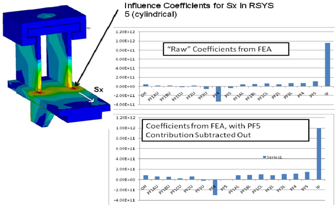
Figure 12.3-6 Influence Coefficients
