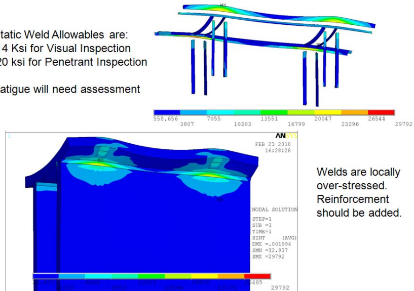
Figure 8.1-4 PF3 Welded Plate to Rib Weld Analysis - Weld Local Stress
