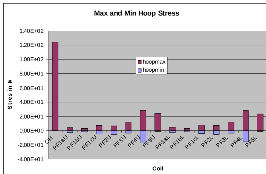
Figure 7.2-1 Early Results for Hoop Stress in the PF Cools
