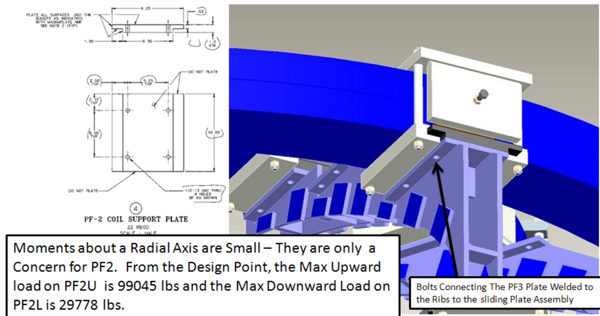
Figure 8.2-2 Sliding Block to Welded Plate Bolting
