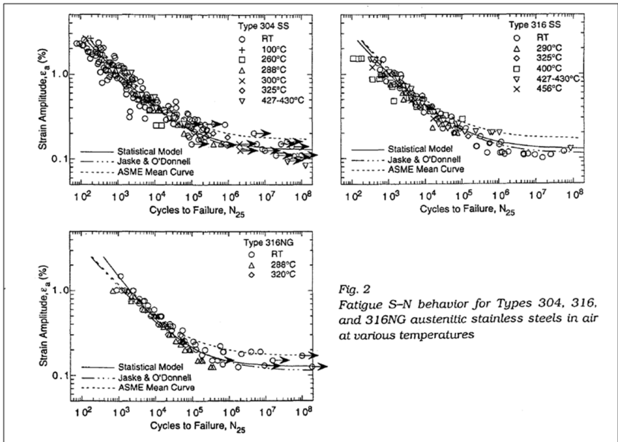
Figure 5.7-1 Fatigue Data for Stainless Steels
