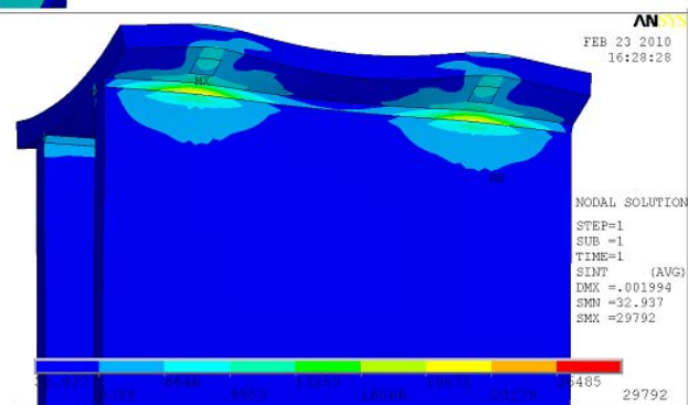
Figure 8.1-1 PF3 Welded Plate to Rib Weld Analysis
