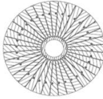
Original TF Bundle 7.9 inch diameter Upgraded TF Bundle 15.7 inch diameter
