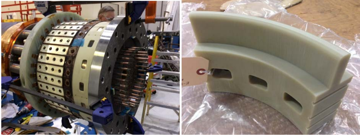
Figure 3.0-1 Machined Crown Segment
