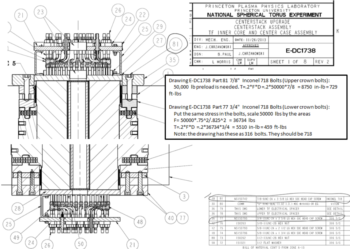
Figure 3a Crown Bolting Requirements
