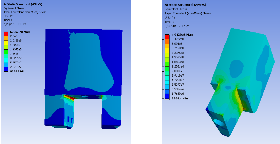
G10 teeth engaging TF Flag
