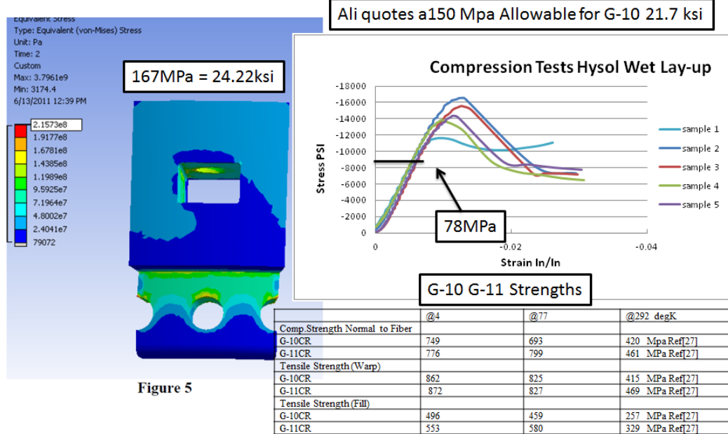
Attachment B Figure 1 Wet Layup Strength Much Lower than G-10
