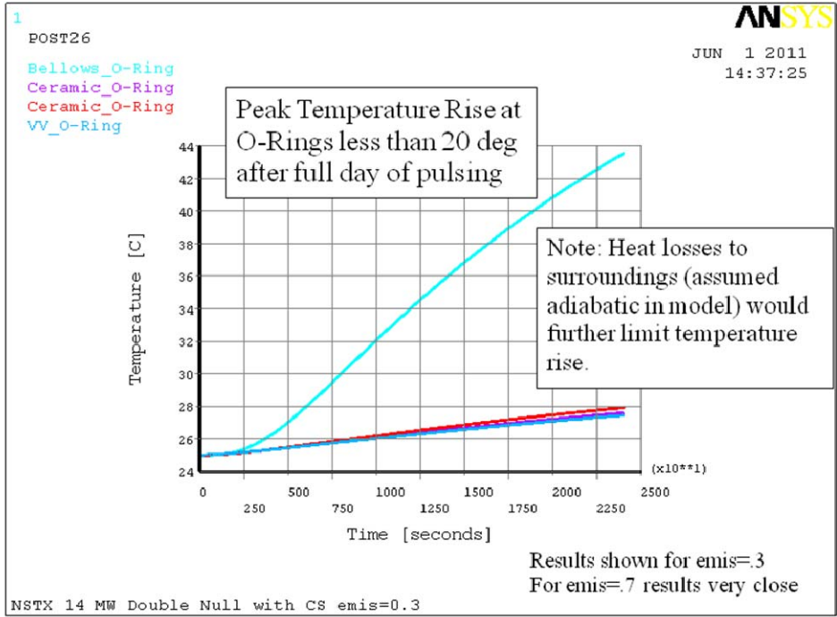
Figure 15 Temperature rise at O-rings for emis=0.3
