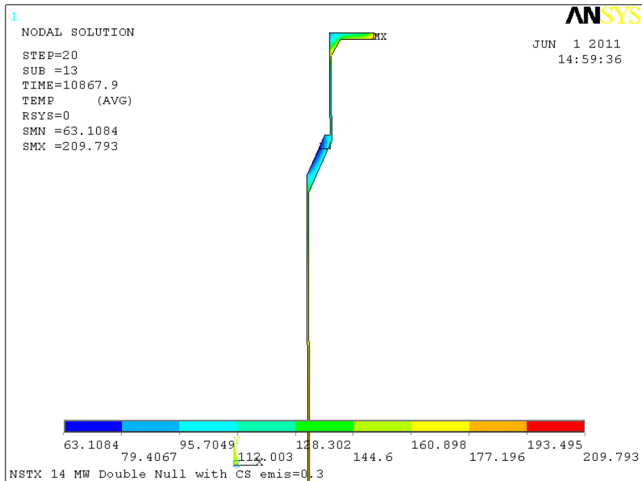
Figure 12 CS Ratched Temperature Distribution, DN, \epsilon=.3
