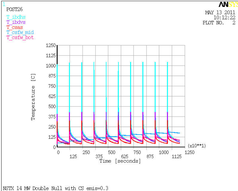
Figure 13 CS Transient Temperature Response, DN, e=.3
