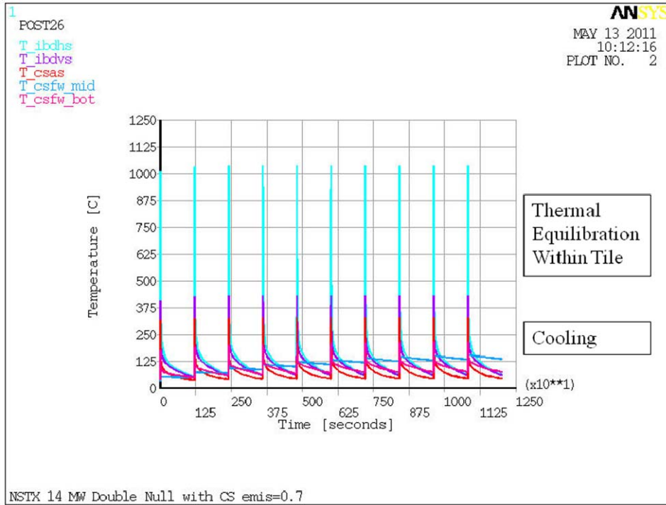
Figure 8 CS Transient Temperature Response, DN, e=0.7
