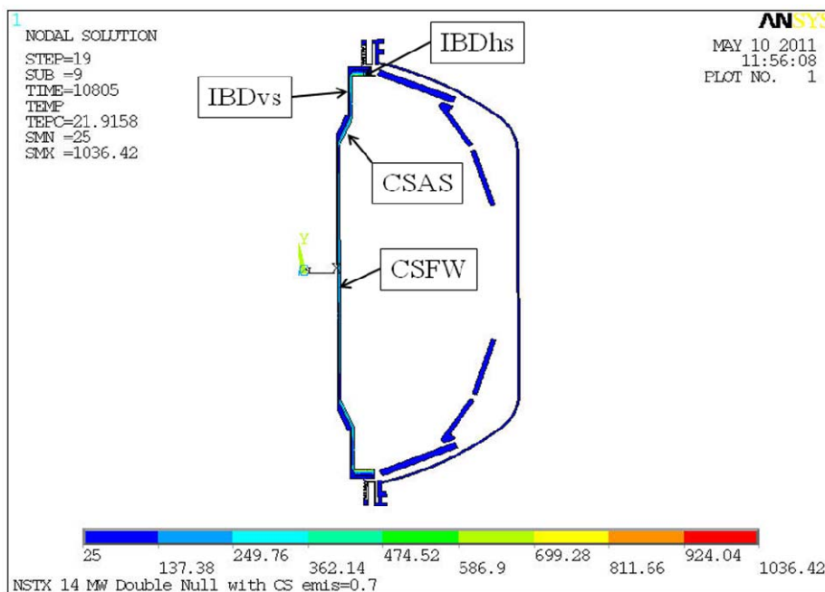
Figure 6 Ratcheted Temperature Distribution DN , e= 0.7
